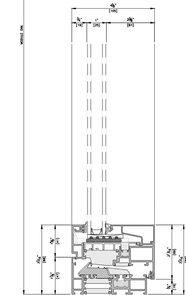
VERTICAL SECTION DETAIL B-B' SCALE : 1/3
