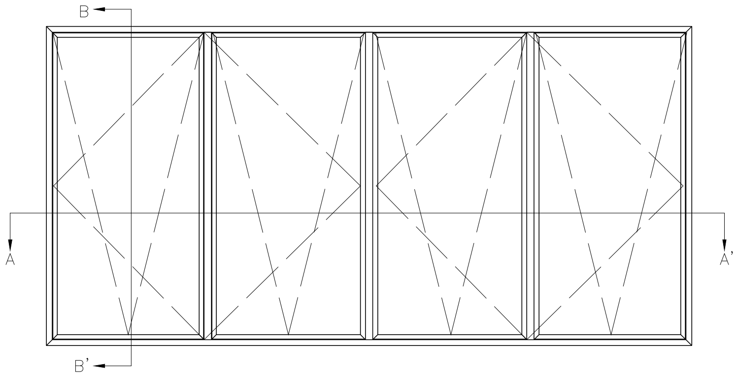
ELEVATION SCALE : 1/30
