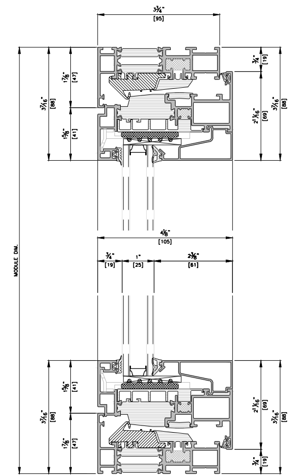
VERTICAL SECTION DETAIL B-B' SCALE : 1/3
