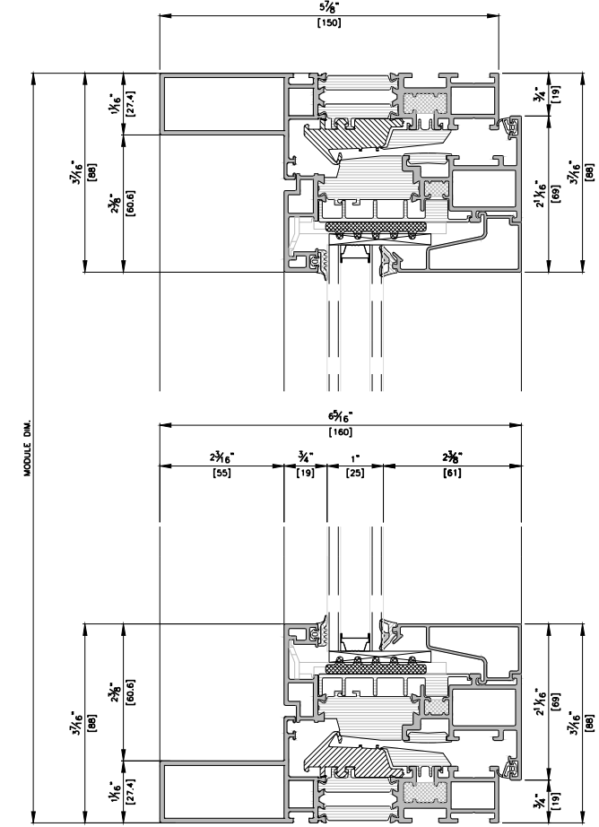
1 VERTICAL SECTION DETAIL B-B' SCALE : 1/3
