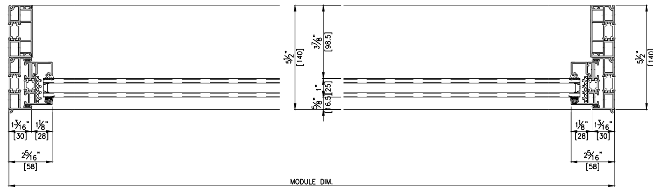
① HORIZONTAL SECTION DETAIL A-A' SCALE : 1/5
