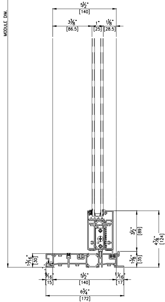
① VERTICAL SECTION DETAIL B-B' SCALE : 1/5
