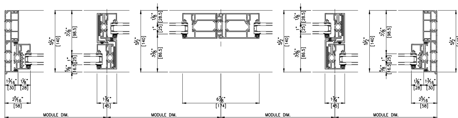
HORIZONTAL SECTION DETAIL A-A' SCALE : 1/5
