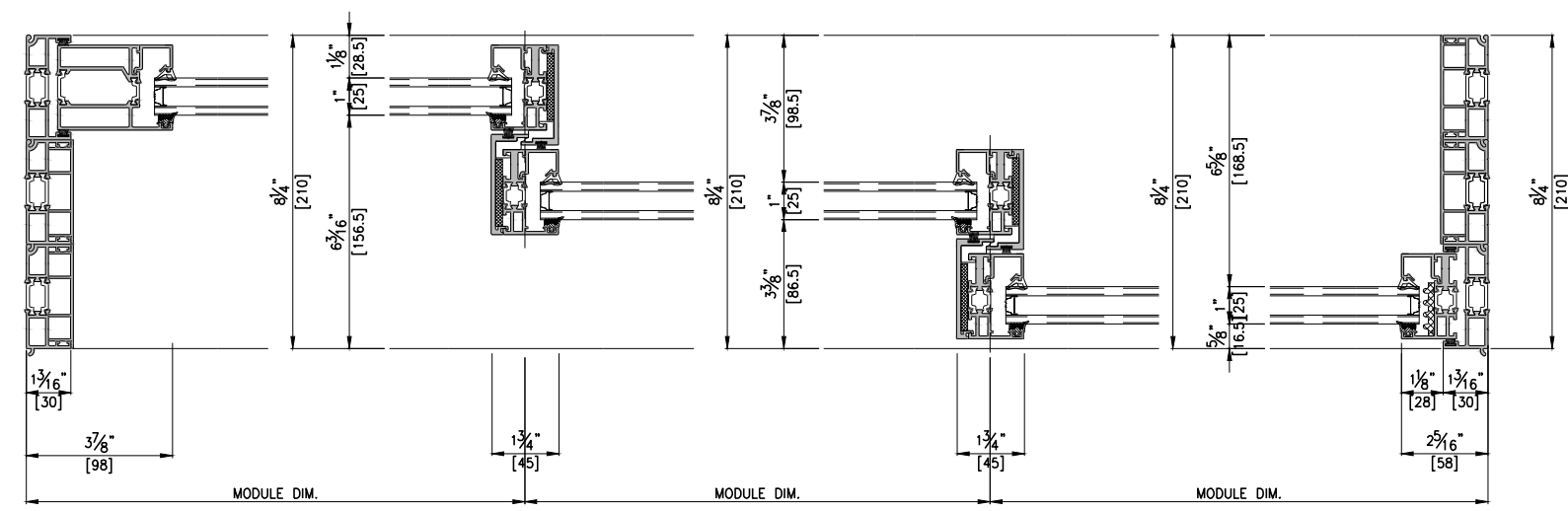
HORIZONTAL SECTION DETAIL A-A' SCALE : 1/5
