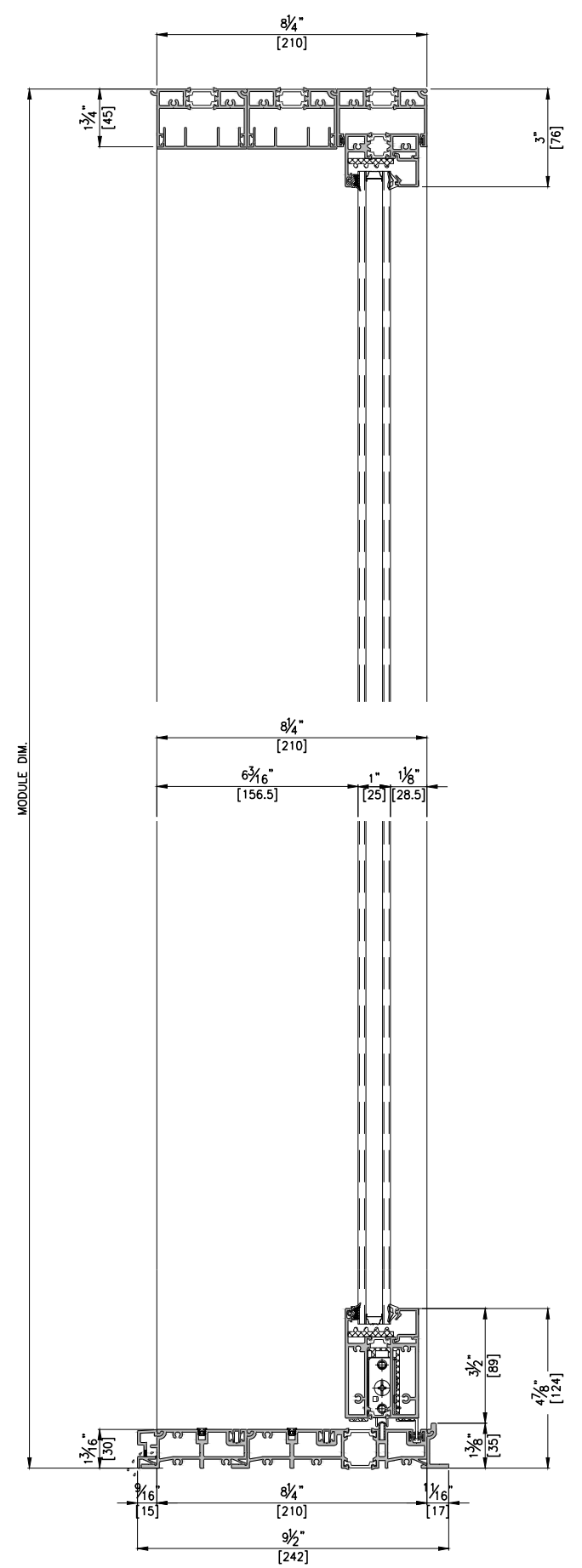
VERTICAL SECTION DETAIL B-B' SCALE : 1/5
