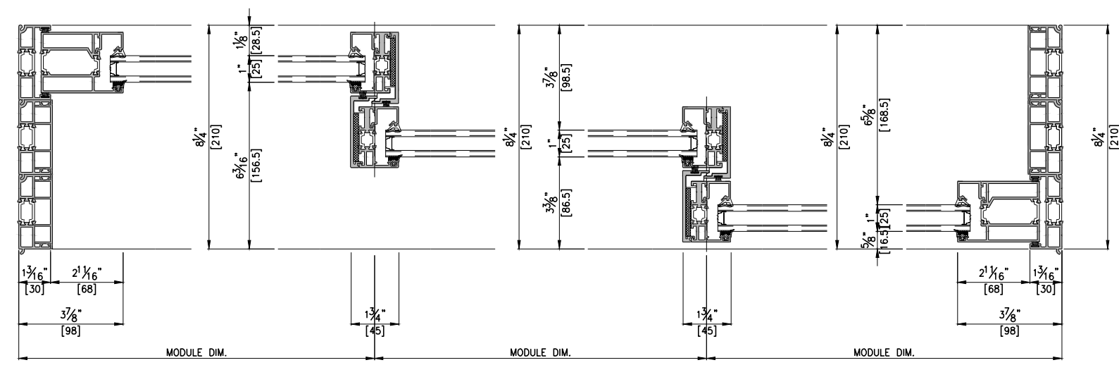
1 HORIZONTAL SECTION DETAIL A-A' SCALE: 1/5
