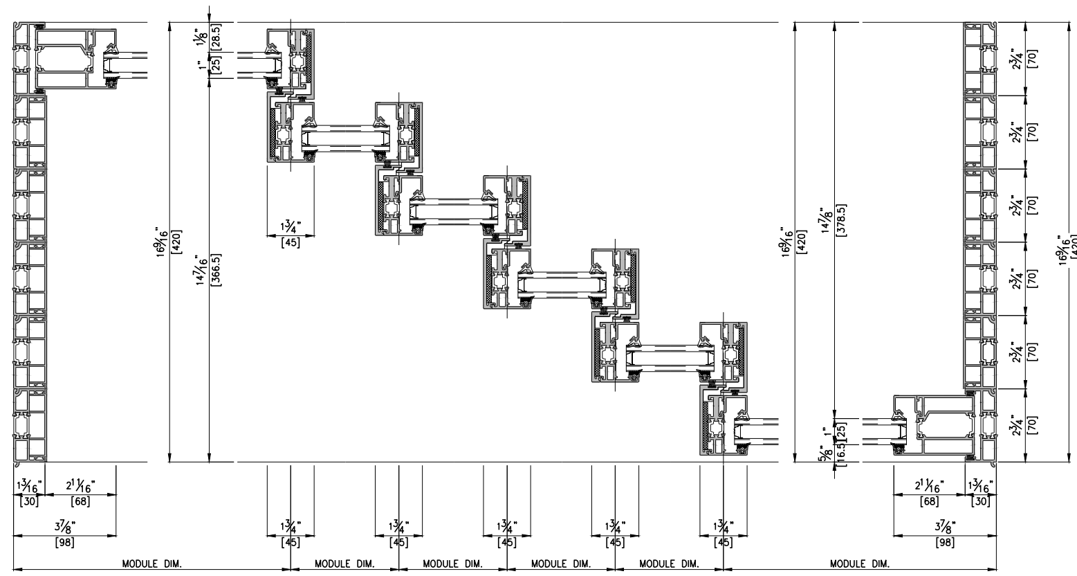
1 HORIZONTAL SECTION DETAIL A-A' SCALE: 1/5
