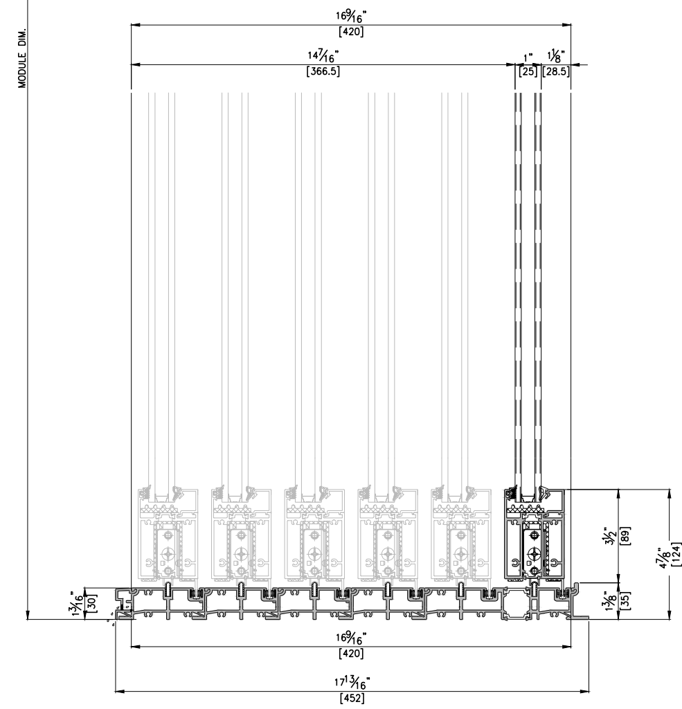
1 VERTICAL SECTION DETAIL B-B' SCALE: 1/5
