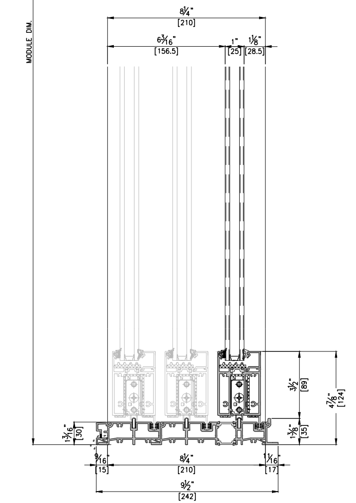
1 VERTICAL SECTION DETAIL B-B' SCALE: 1/5
