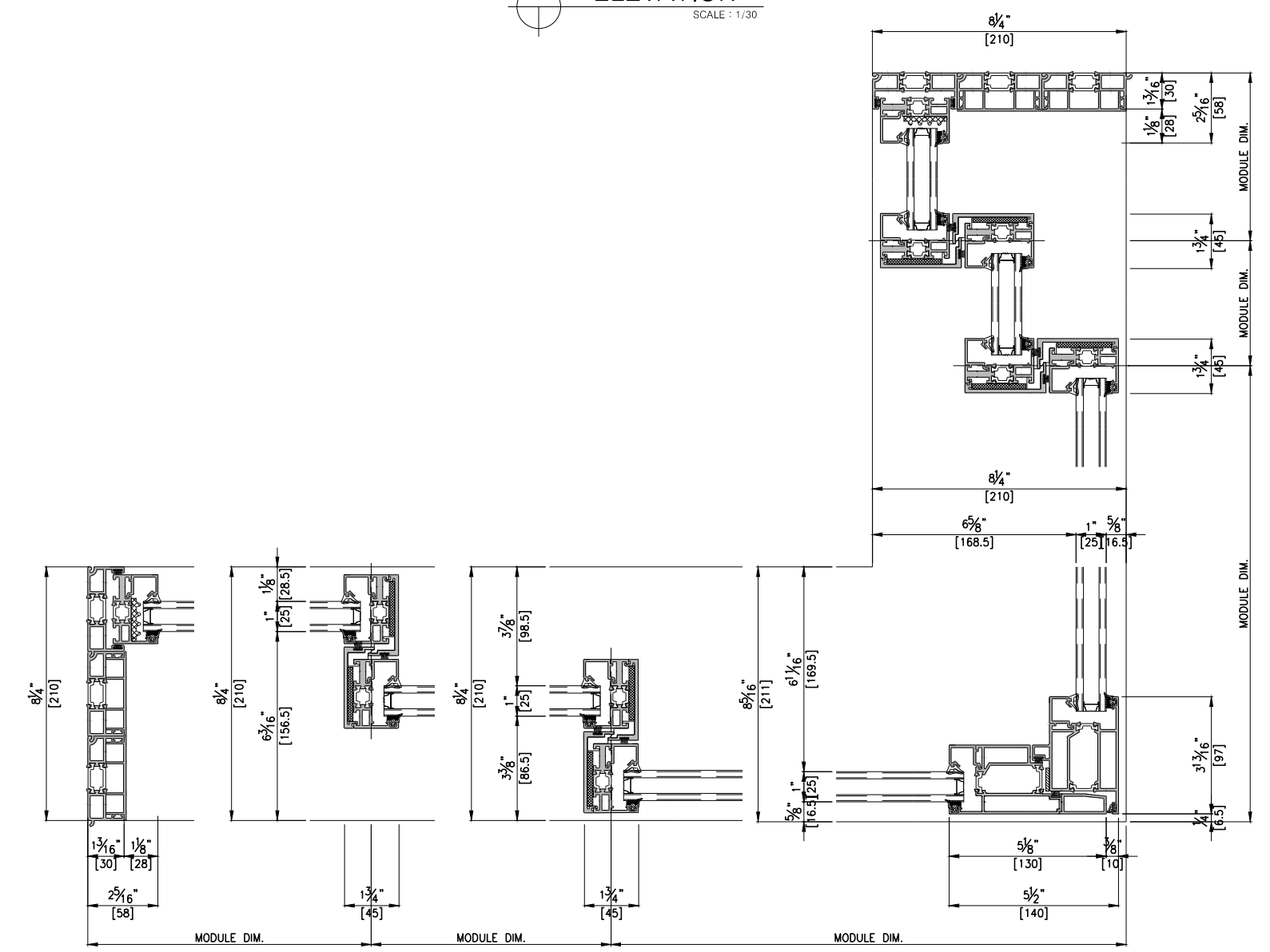
1 HORIZONTAL SECTION DETAIL A-A' SCALE: 1/5
