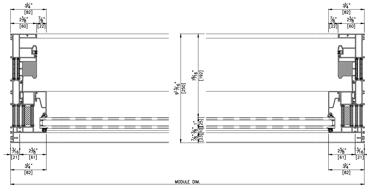
HORIZONTAL SECTION DETAIL A-A' SCALE : 1/5
