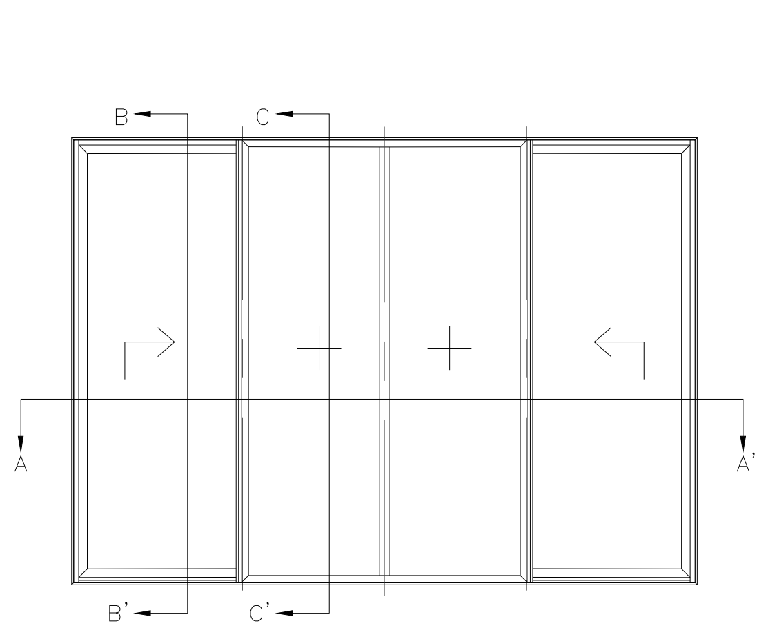
ELEVATION SCALE : 1/30
