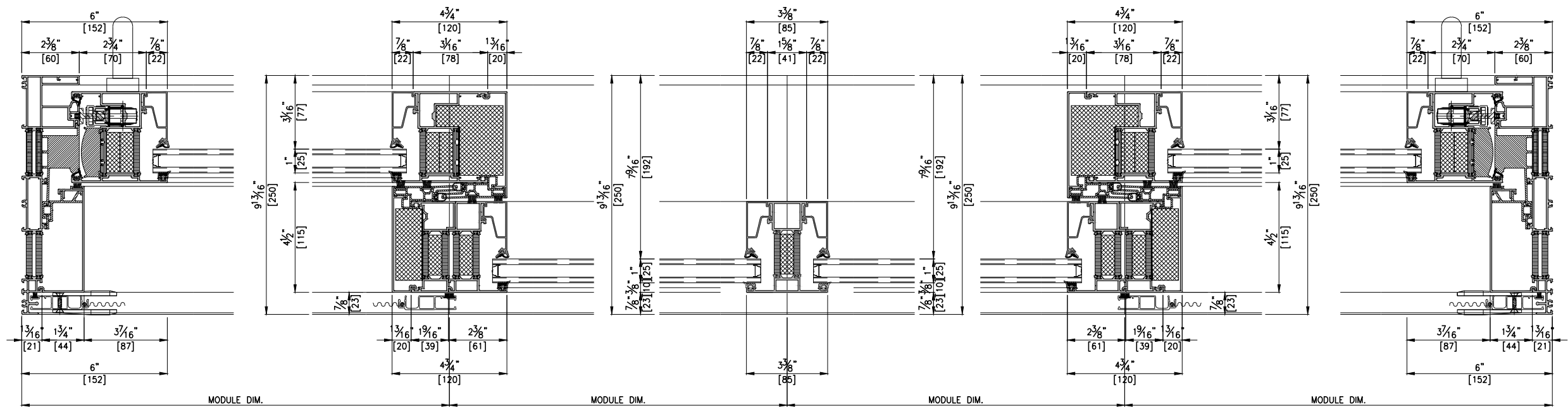
HORIZONTAL SECTION DETAIL A-A' SCALE : 1/5
