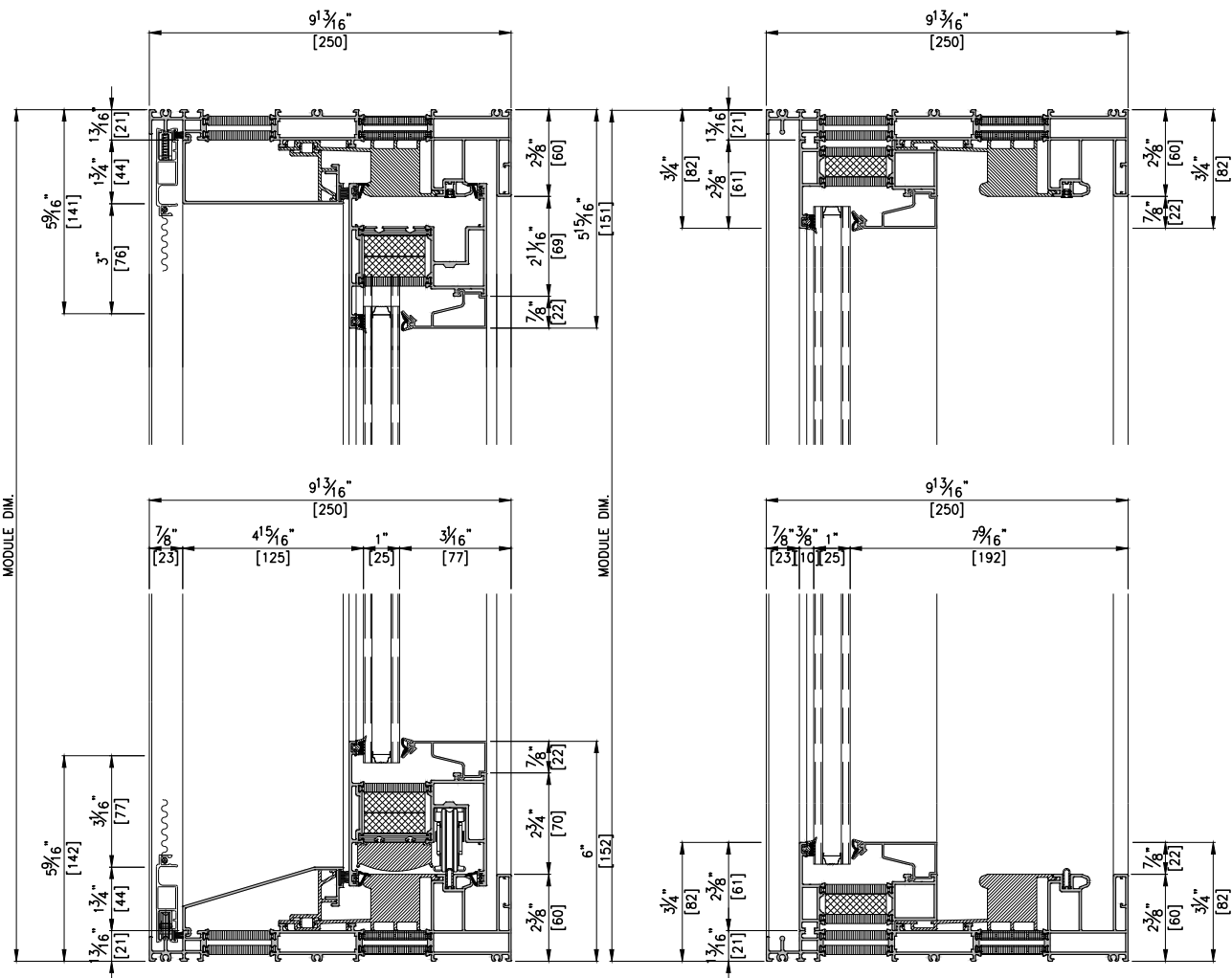
VERTICAL SECTION DETAIL B-B' SCALE : 1/5
