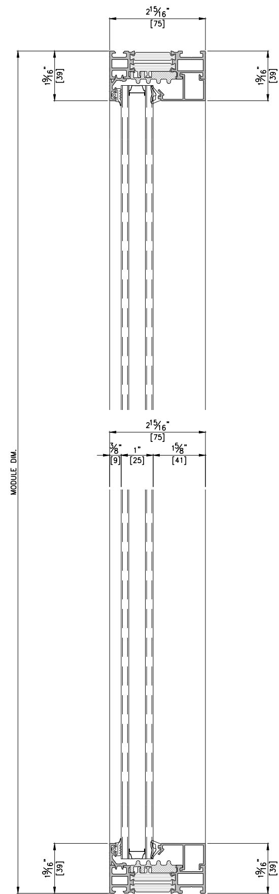
1 VERTICAL SECTION DETAIL B-B' SCALE : 1/3
