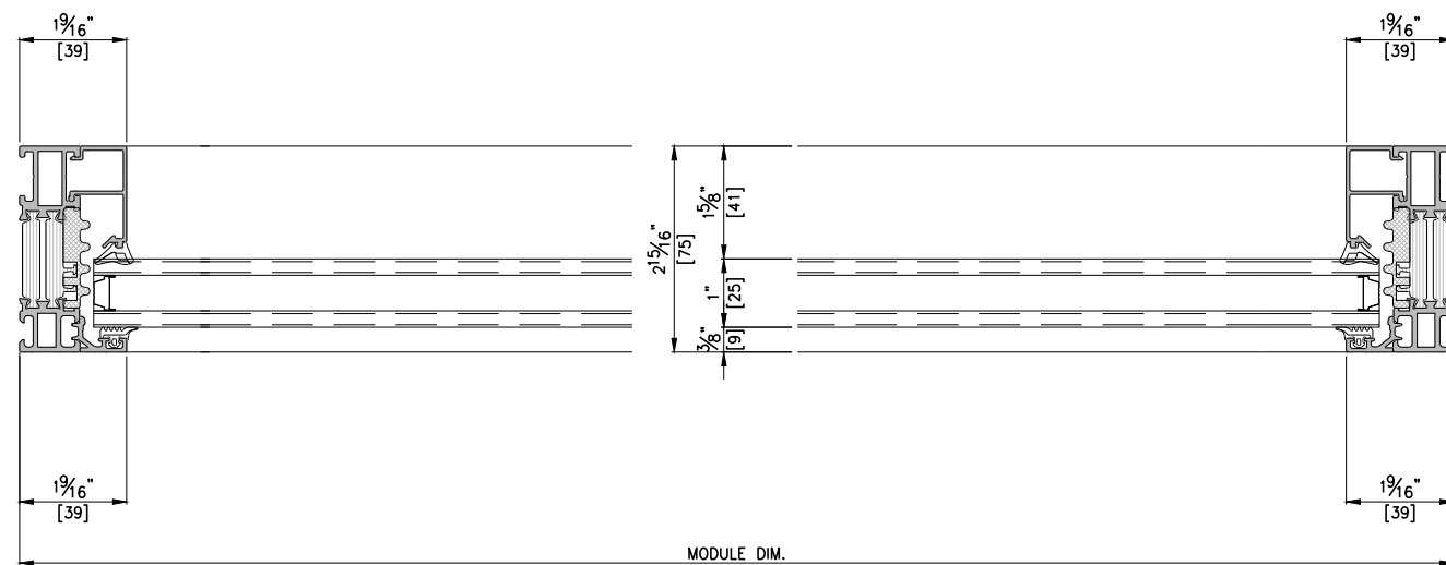
1 HORIZONTAL SECTION DETAIL A-A' SCALE : 1/3
