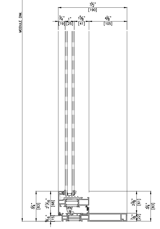
VERTICAL SECTION DETAIL B-B' SCALE : 1/5
