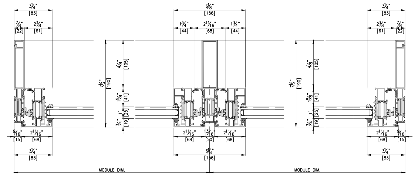
HORIZONTAL SECTION DETAIL A-A' SCALE : 1/5
