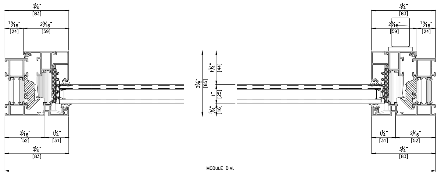
1 HORIZONTAL SECTION DETAIL A-A' SCALE : 1/3
