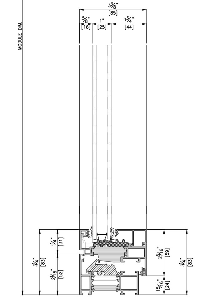
1 VERTICAL SECTION DETAIL B-B' SCALE : 1/3
