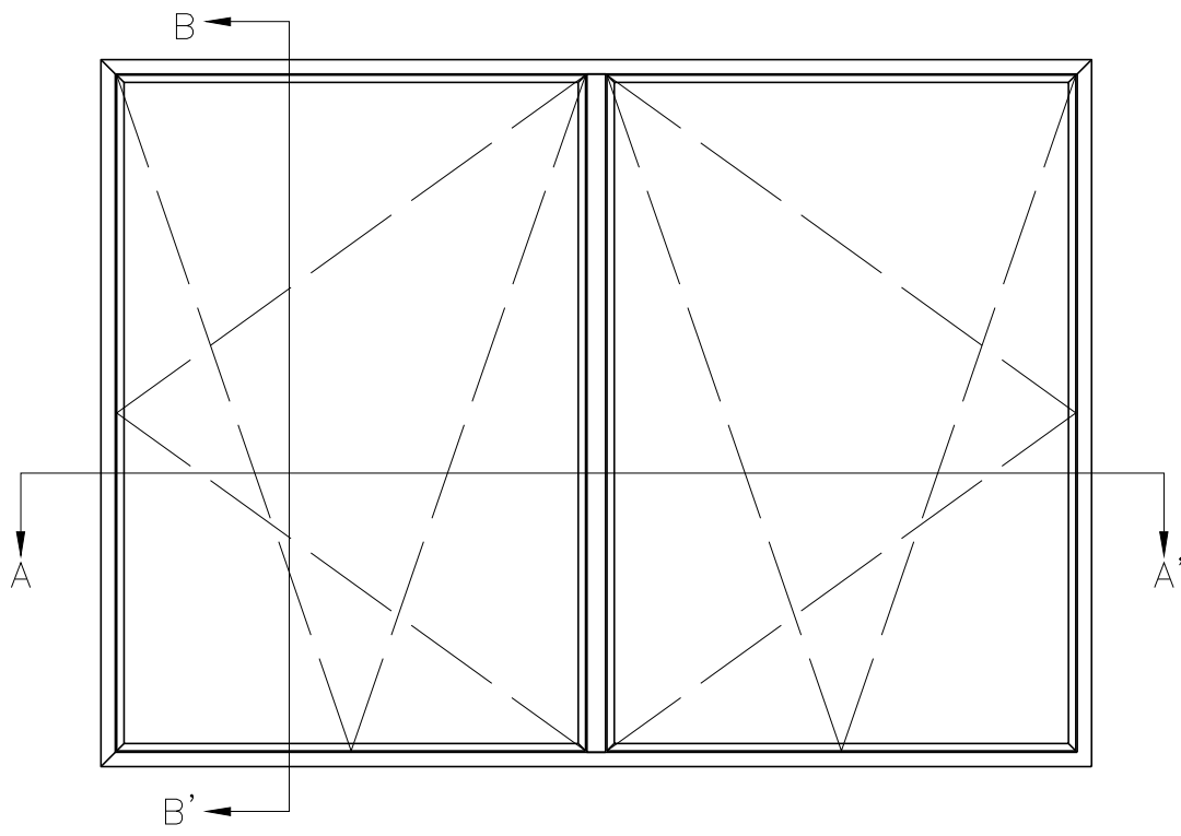
1 ELEVATION SCALE : 1/30
