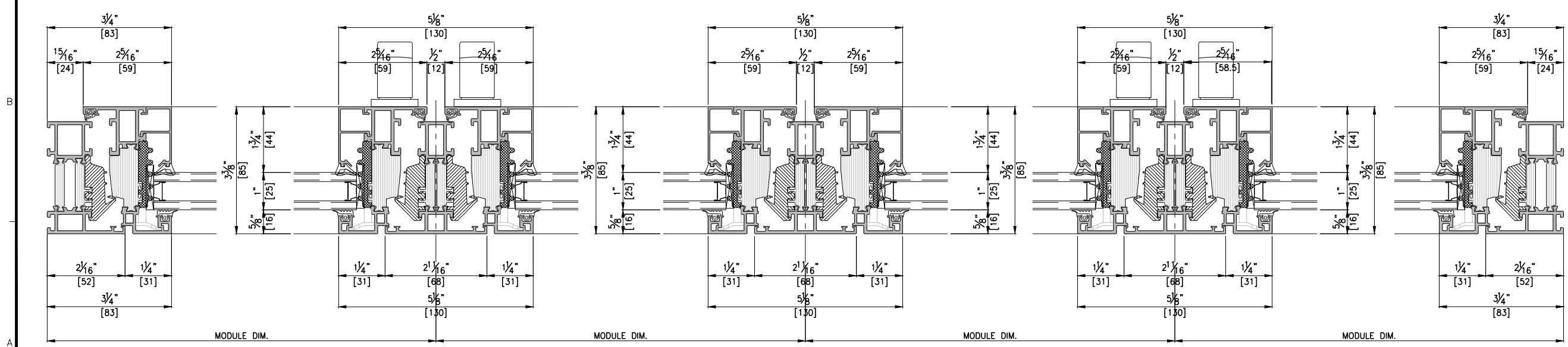
HORIZONTAL SECTION DETAIL A-A' SCALE : 1/3
