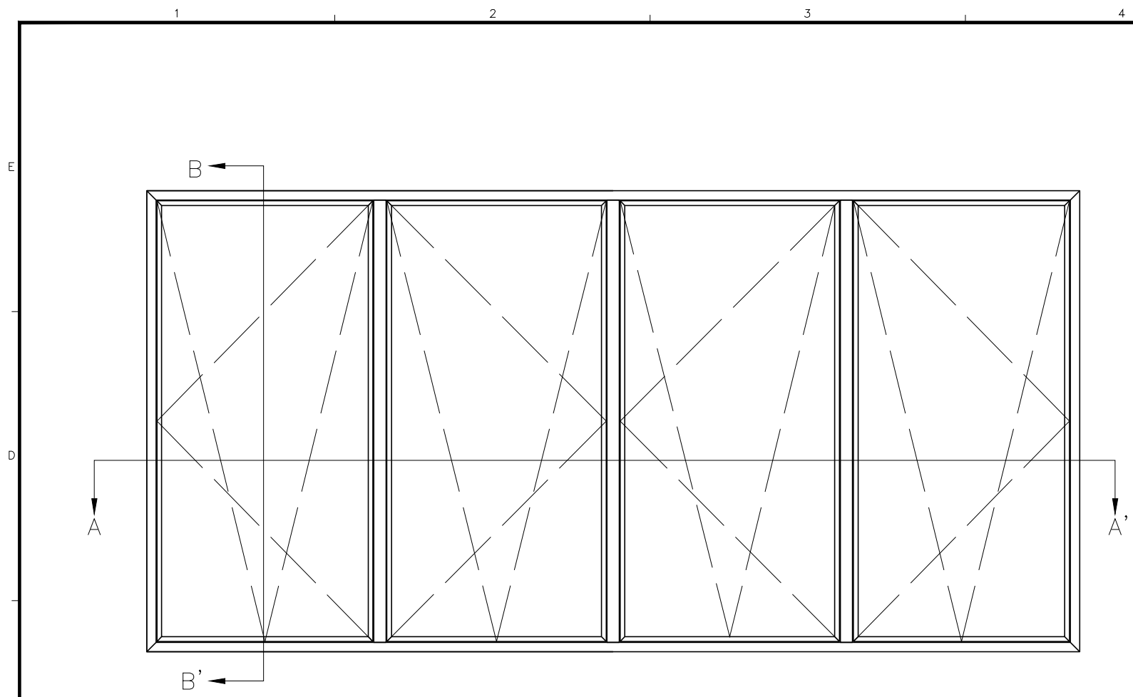
ELEVATION SCALE : 1/30
