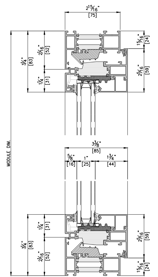
VERTICAL SECTION DETAIL B-B' SCALE : 1/3
