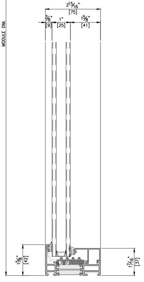
VERTICAL SECTION DETAIL C-C' SCALE : 1/3
