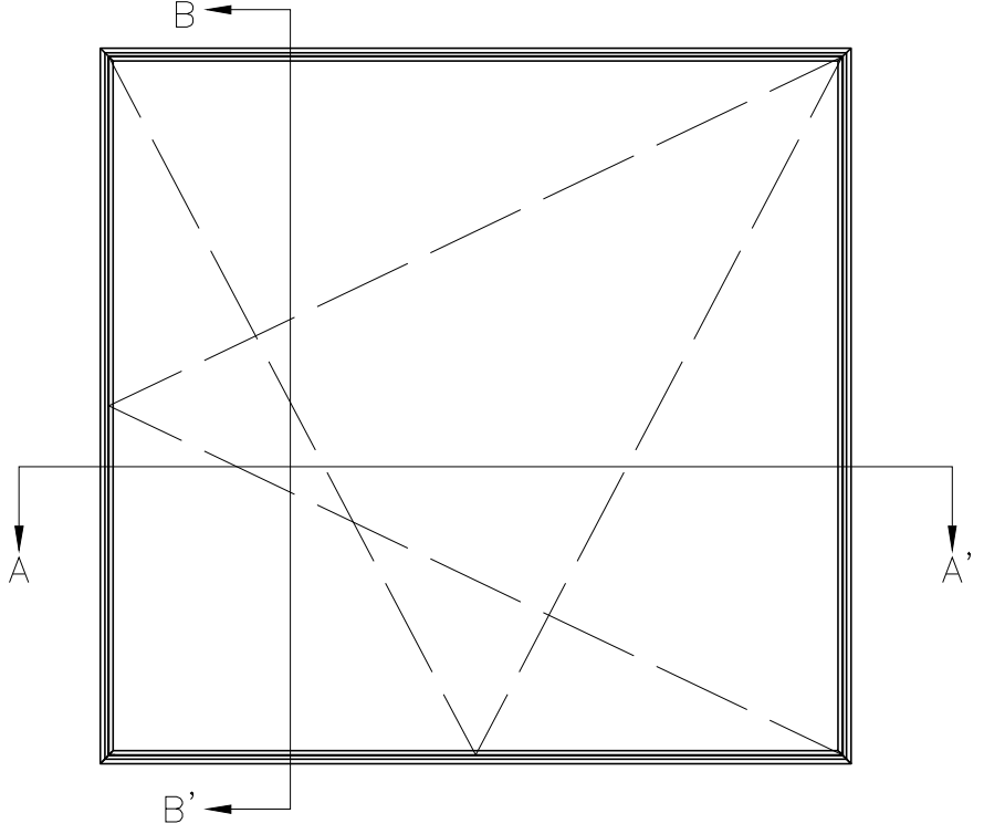
ELEVATION SCALE : 1/30
