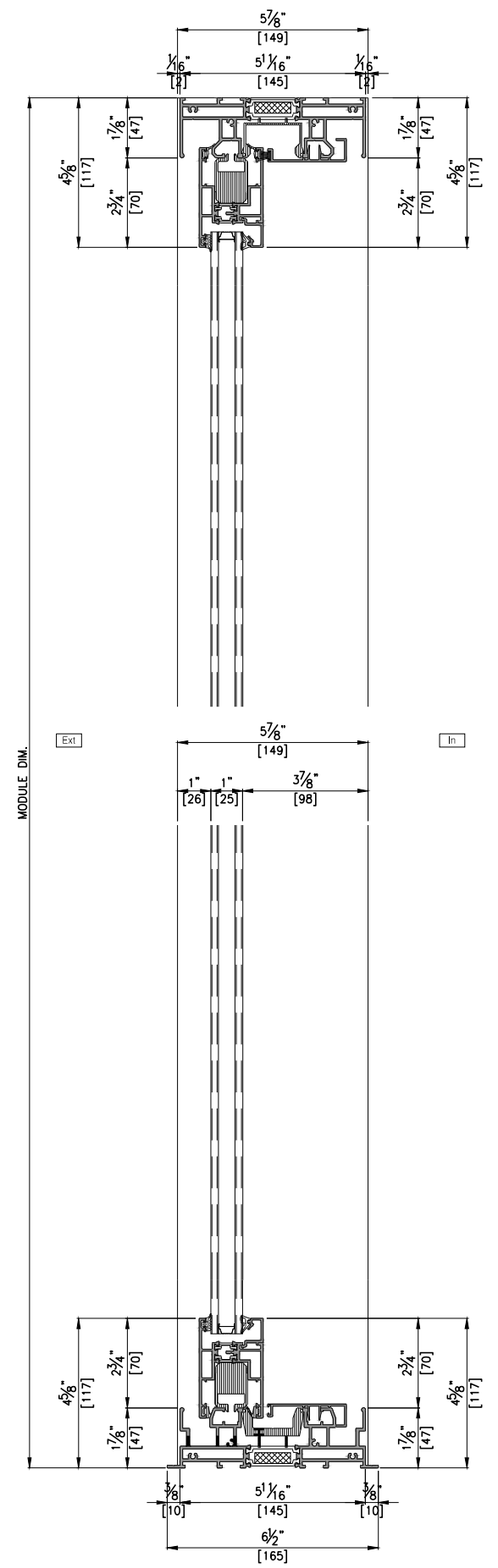
VERTICAL SECTION DETAIL B-B' SCALE : 1/5
