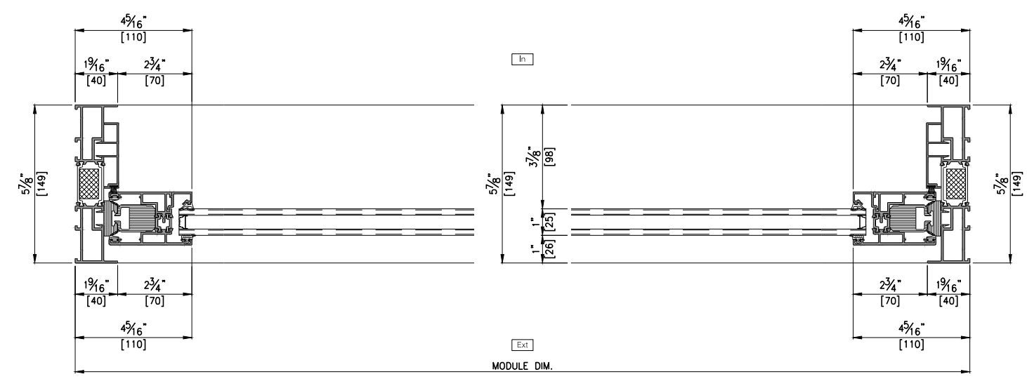
HORIZONTAL SECTION DETAIL A-A'
