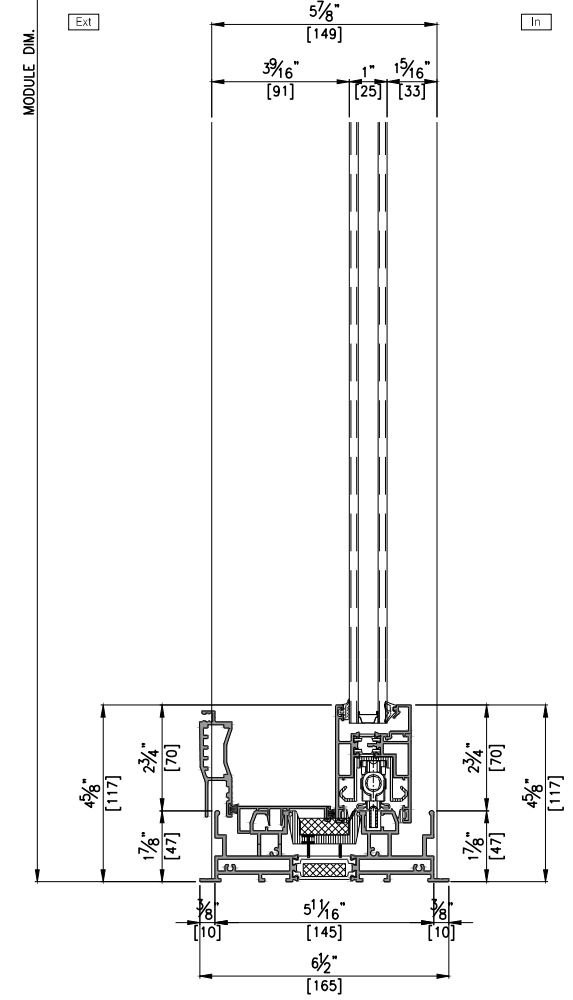
VERTICAL SECTION DETAIL B-B' SCALE : 1/5
