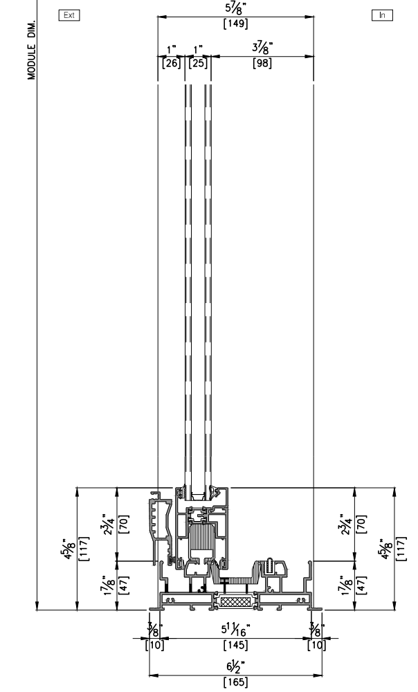
VERTICAL SECTION DETAIL C-C' SCALE : 1/5
