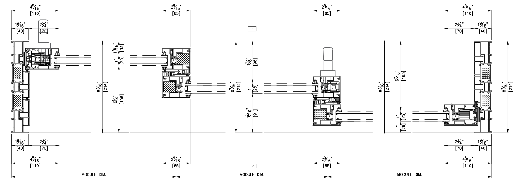
HORIZONTAL SECTION DETAIL A-A' SCALE : 1/5
