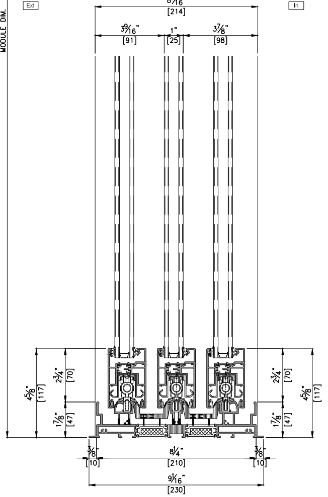
VERTICAL SECTION DETAIL B-B' SCALE : 1/5
