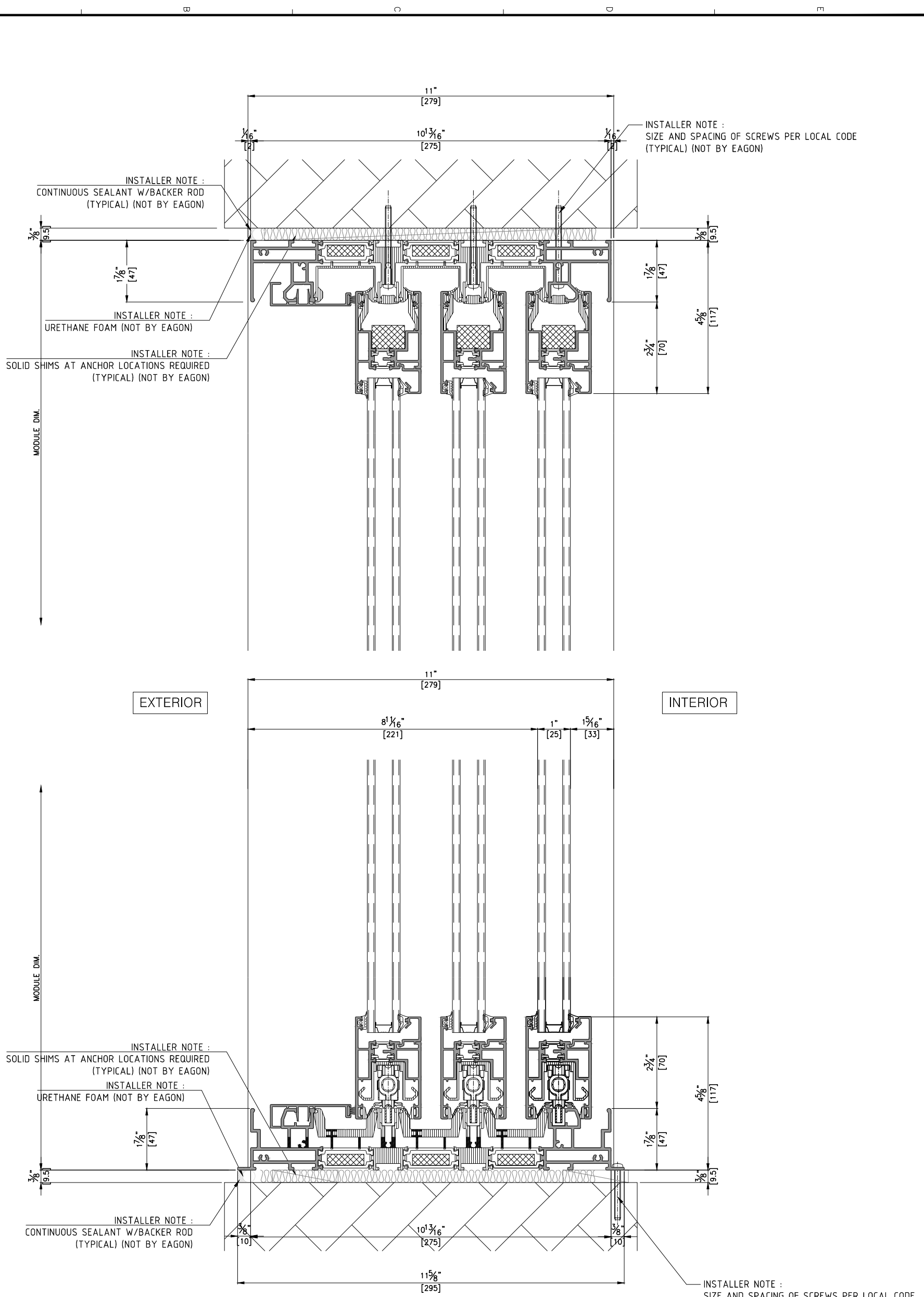
VERTICAL SECTION DETAIL
