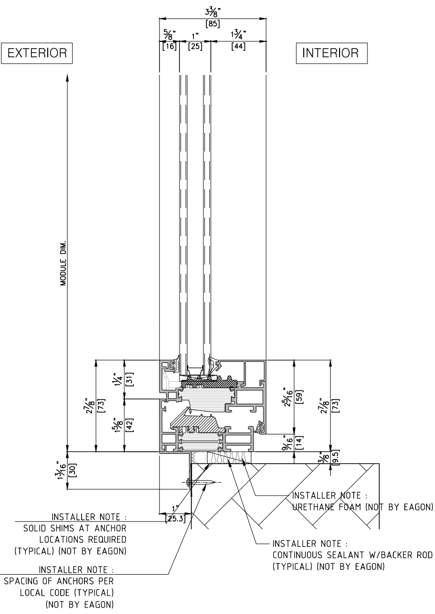
1 VERTICAL SECTION DETAIL SCALE: 1/3
