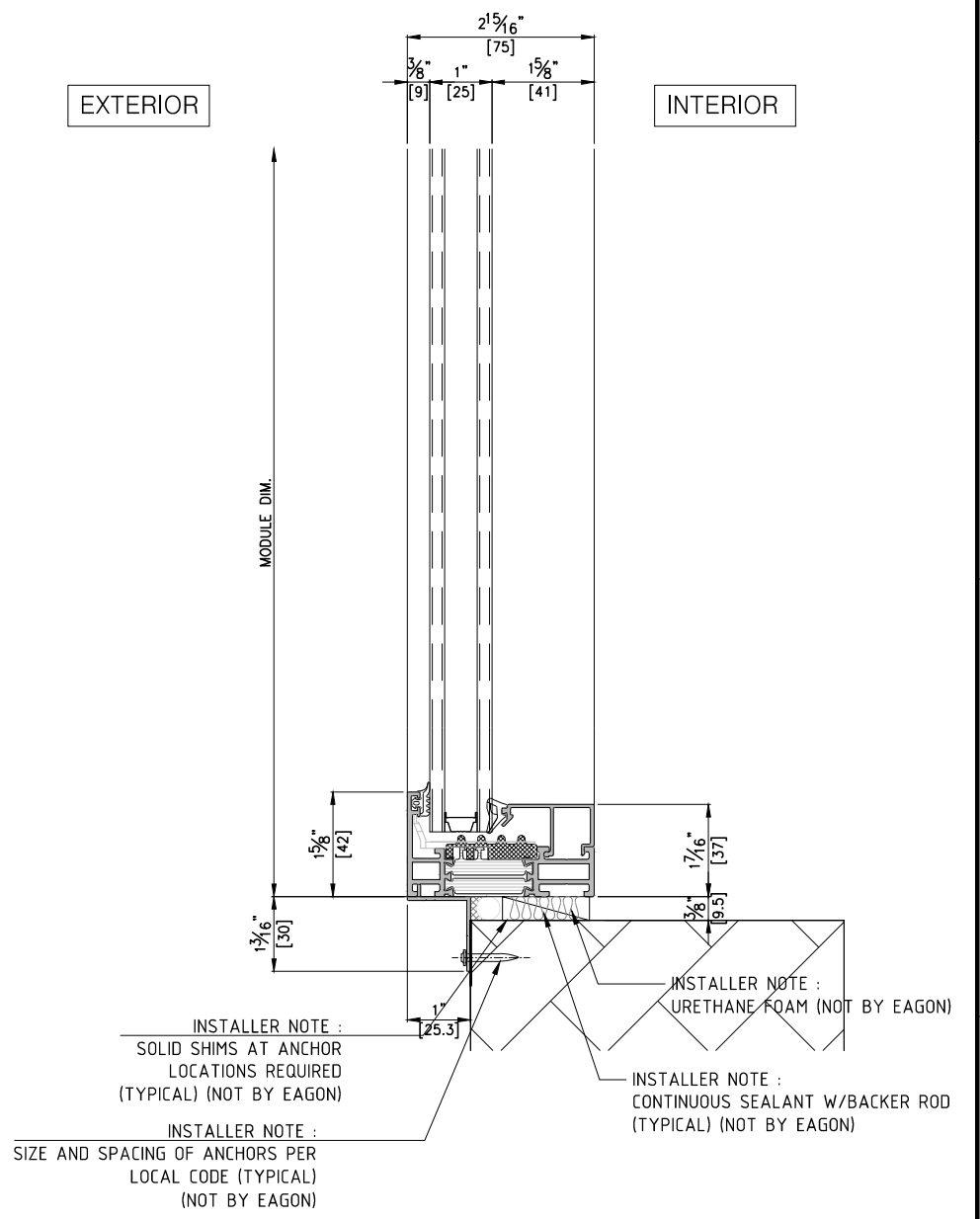
2 VERTICAL SECTION DETAIL SCALE: 1/3
