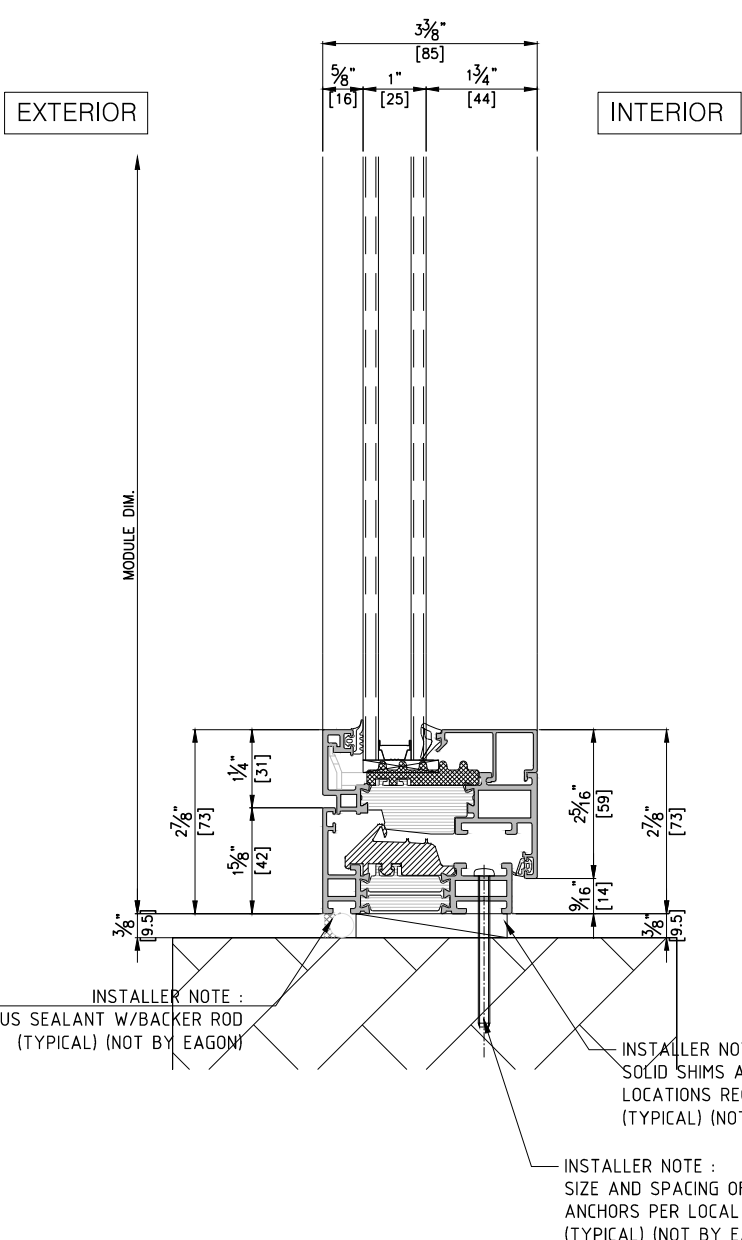
1 VERTICAL SECTION DETAIL SCALE: 1/3
