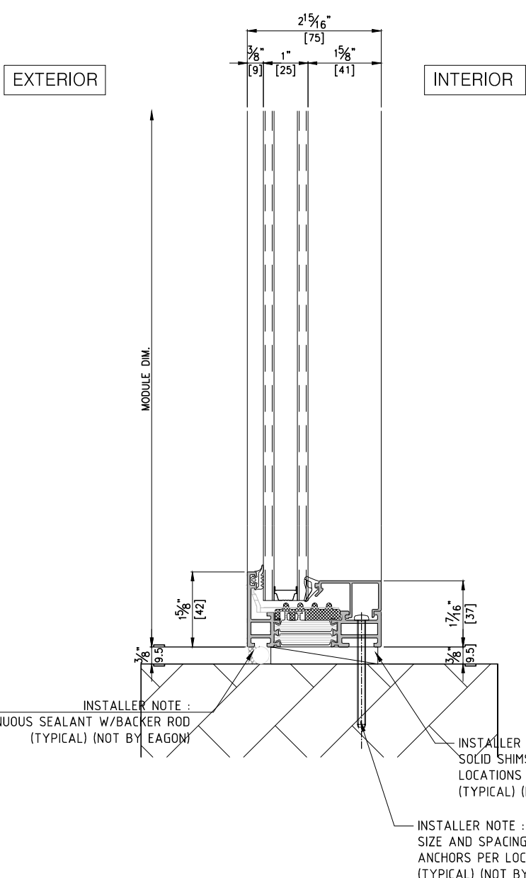
2 VERTICAL SECTION DETAIL SCALE: 1/3
