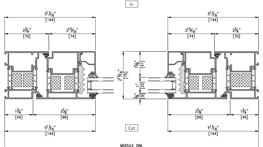
HORIZONTAL SECTION DETAIL A-A' SCALE : 1/3
