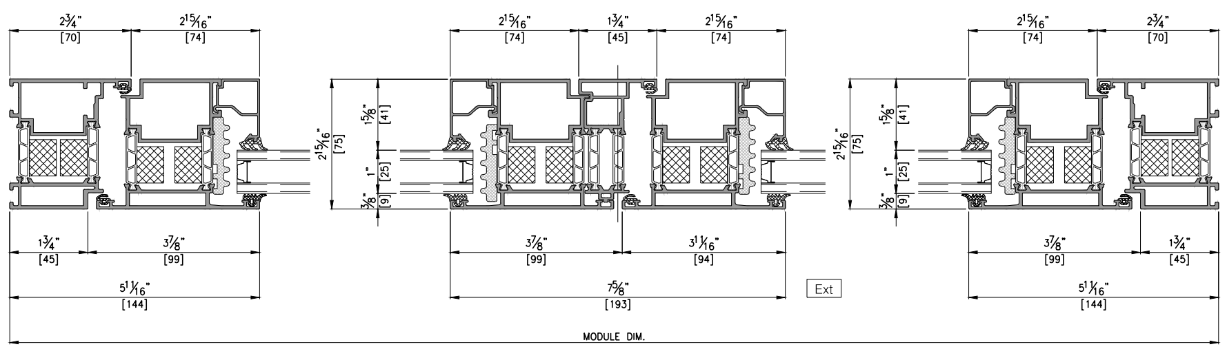
HORIZONTAL SECTION DETAIL A-A' SCALE: 1/3
