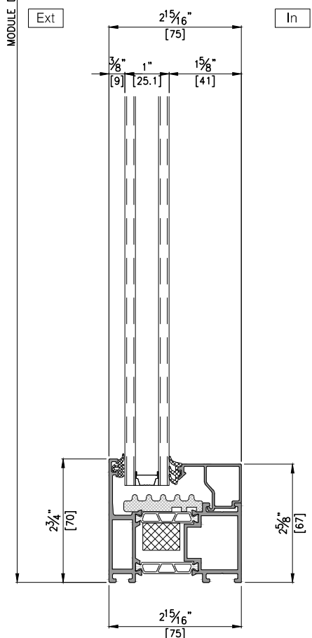
VERTICAL SECTION DETAIL B-B' SCALE: 1/3
