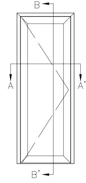
ELEVATION SCALE : 1/30
