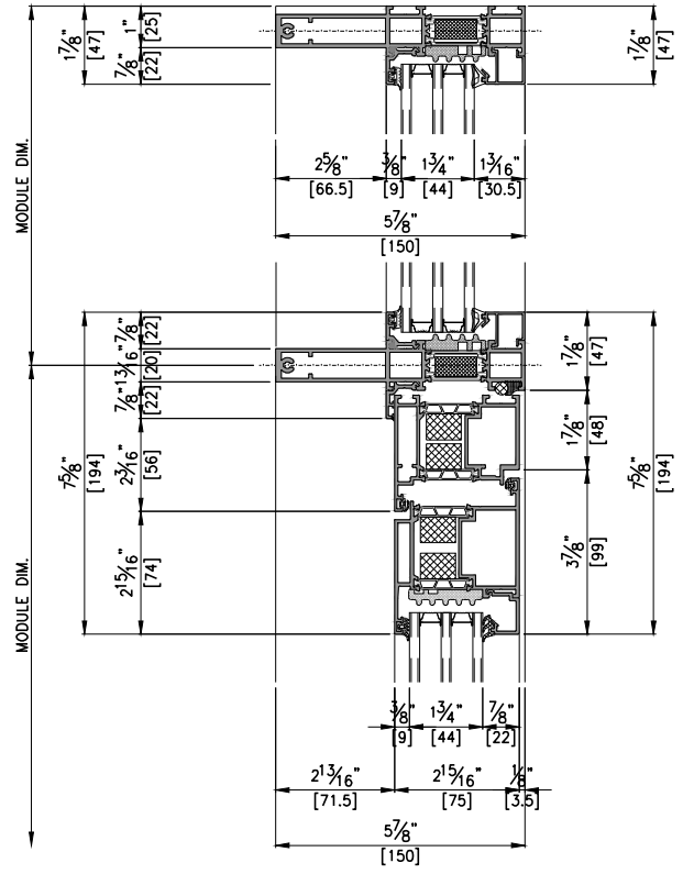
VERTICAL SECTION DETAIL
