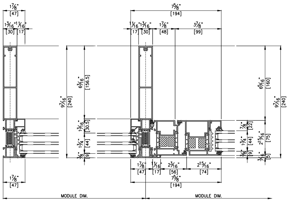
HORIZONTAL SECTION DETAIL
