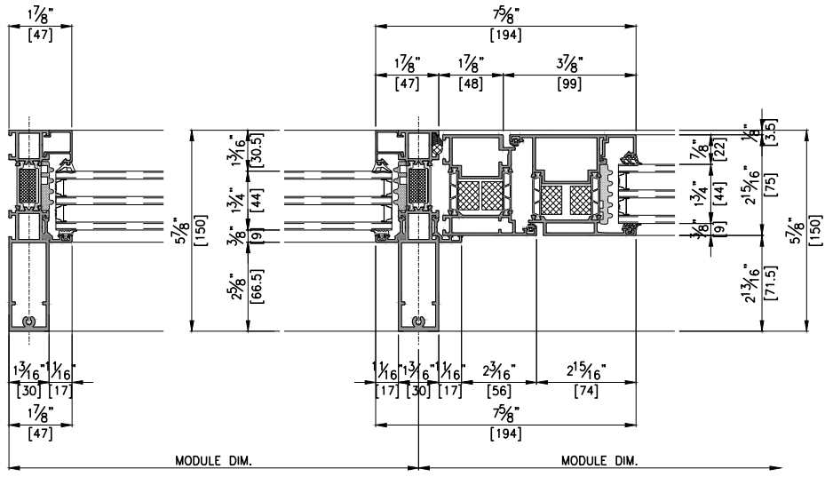
HORIZONTAL SECTION DETAIL
