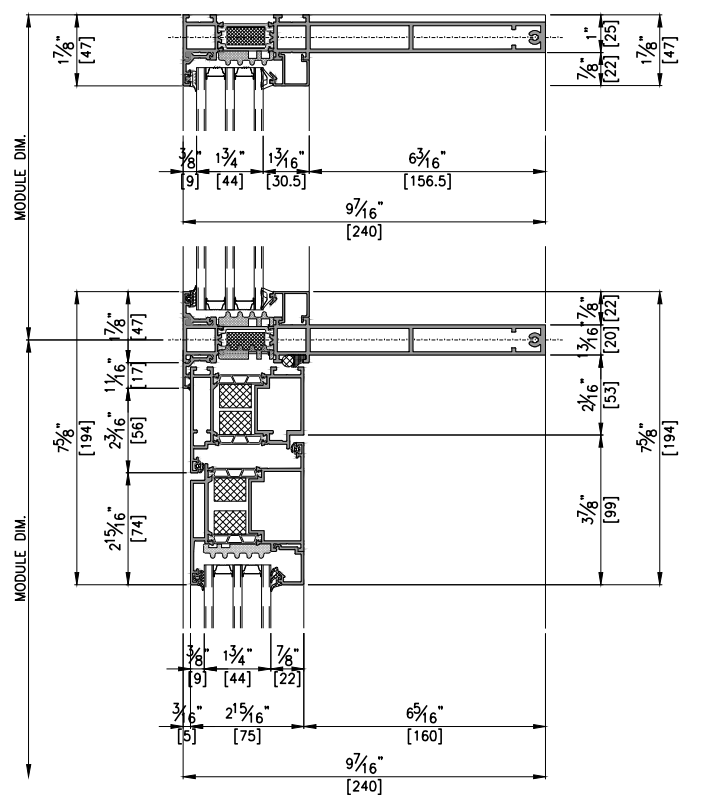
VERTICAL SECTION DETAIL
