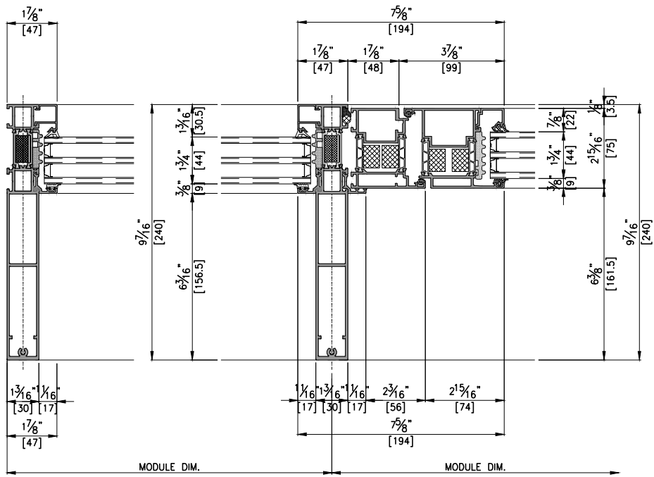
HORIZONTAL SECTION DETAIL
