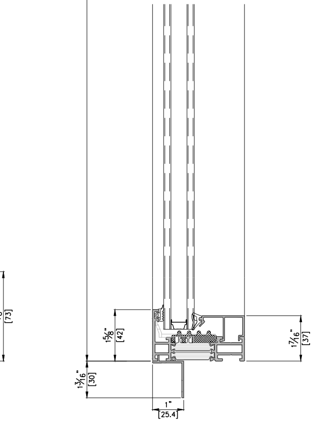
VERTICAL SECTION DETAIL C-C' SCALE : 1/3
