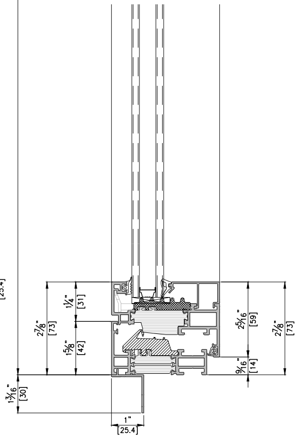
VERTICAL SECTION DETAIL B-B' SCALE : 1/3
