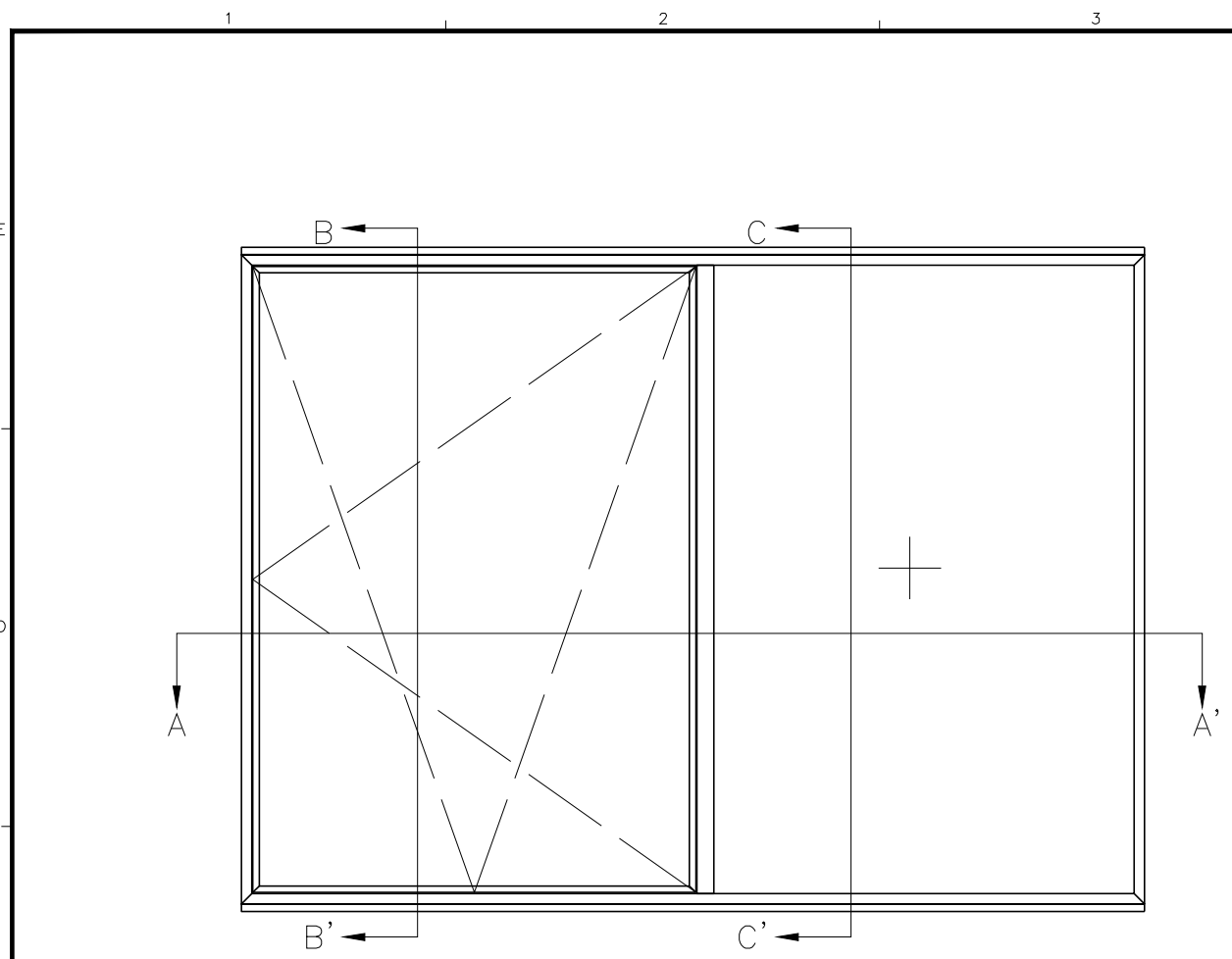
ELEVATION SCALE : 1/30
