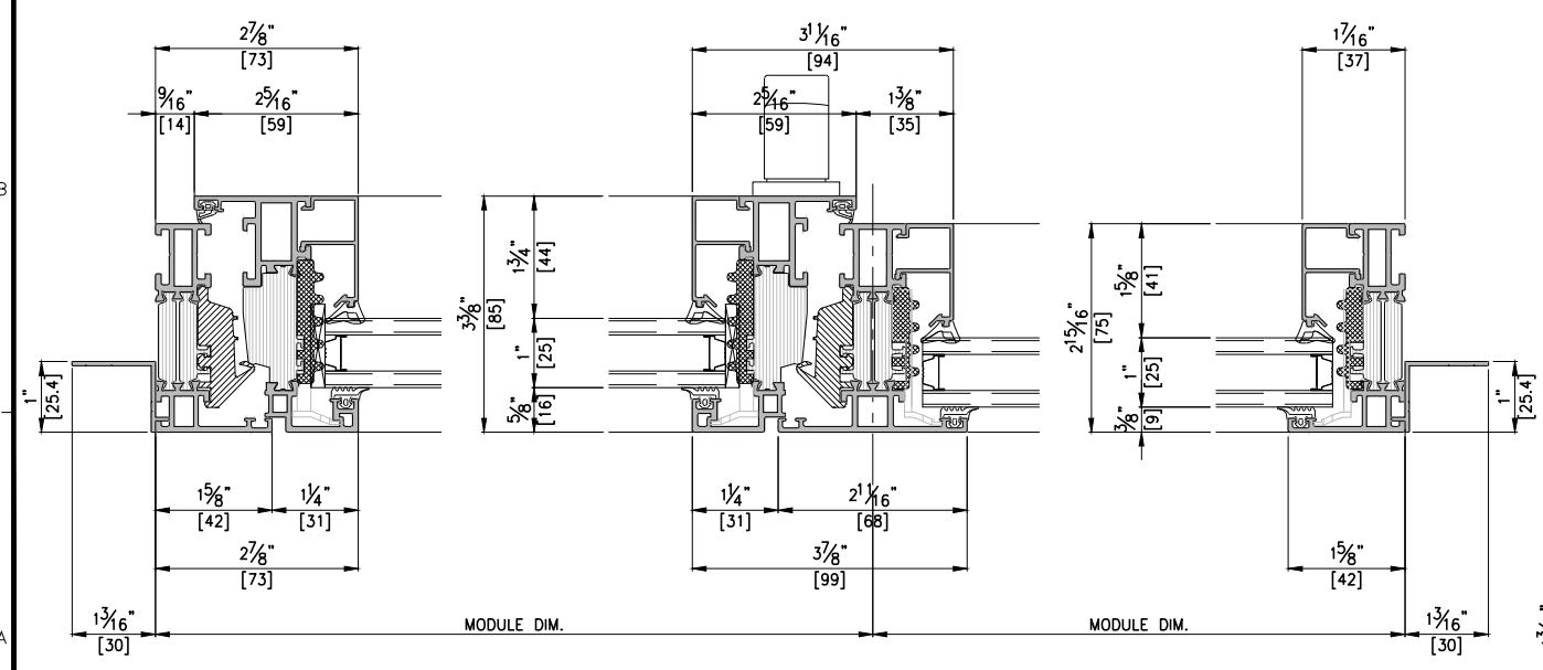
HORIZONTAL SECTION DETAIL A-A' SCALE : 1/3
